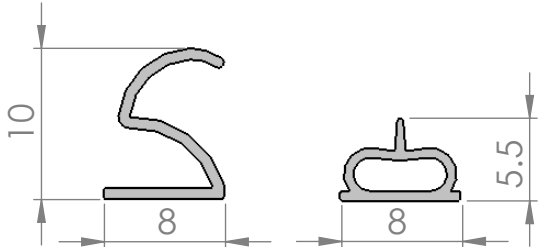
MF-T8 ADHESIVE TAPE CLEAR SIDE TO SEAL PAPER SIDE TO SUBSTRATE
